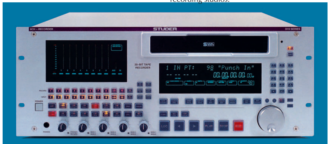
Fig. 2: Front of the STUDER V-EIGHT unit.
